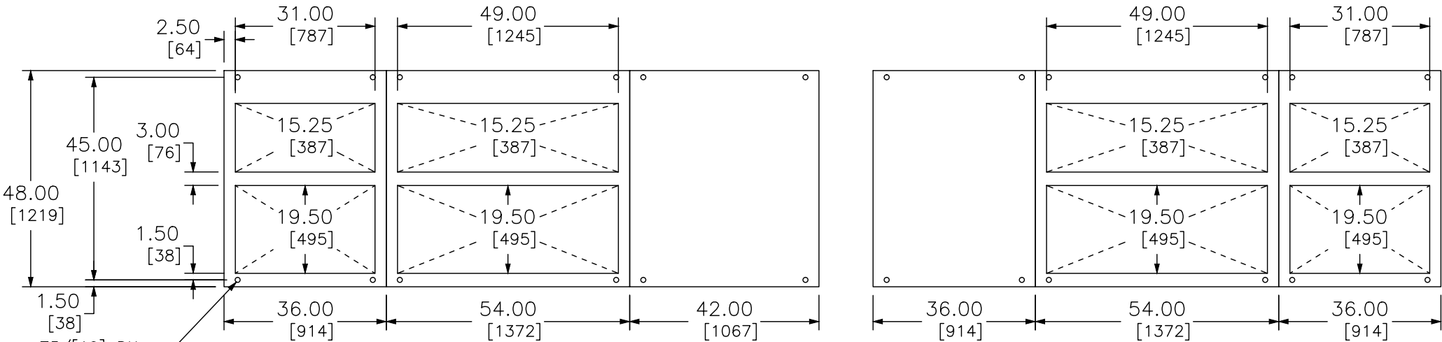
FLOOR PLAN — FRONT
